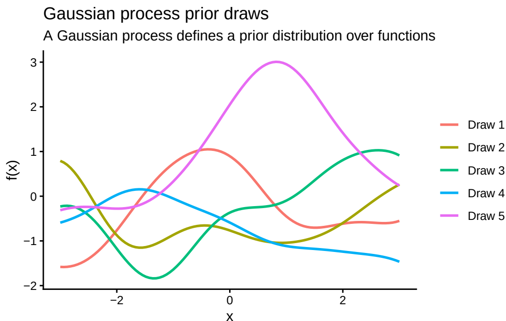
Figure 9.2: Draws from a Gaussian process prior.
