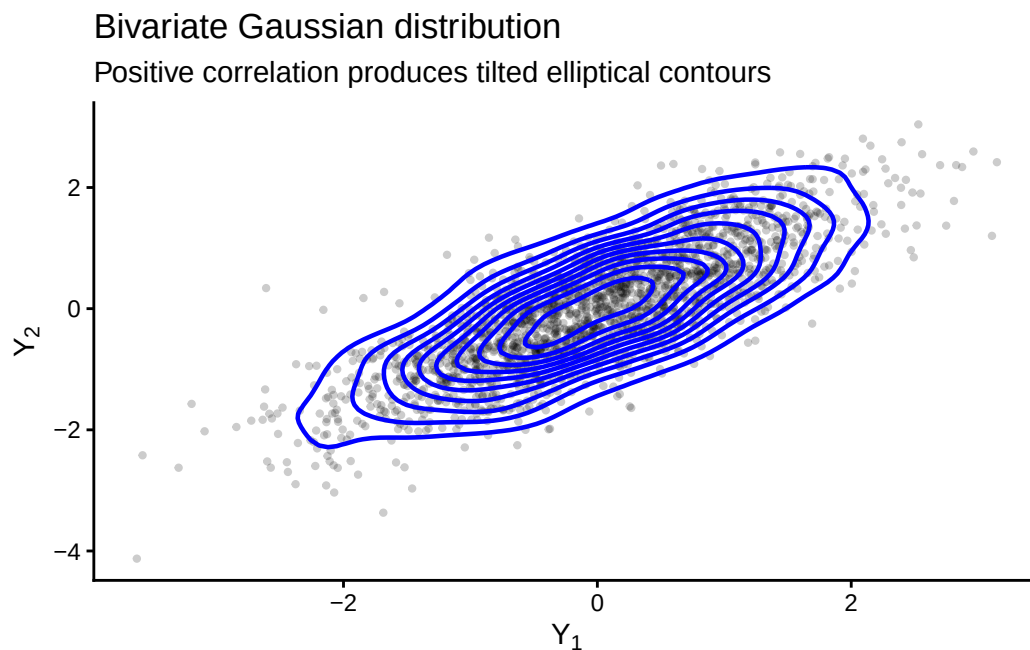
Figure 7.1: A bivariate Gaussian distribution with positive correlation.
