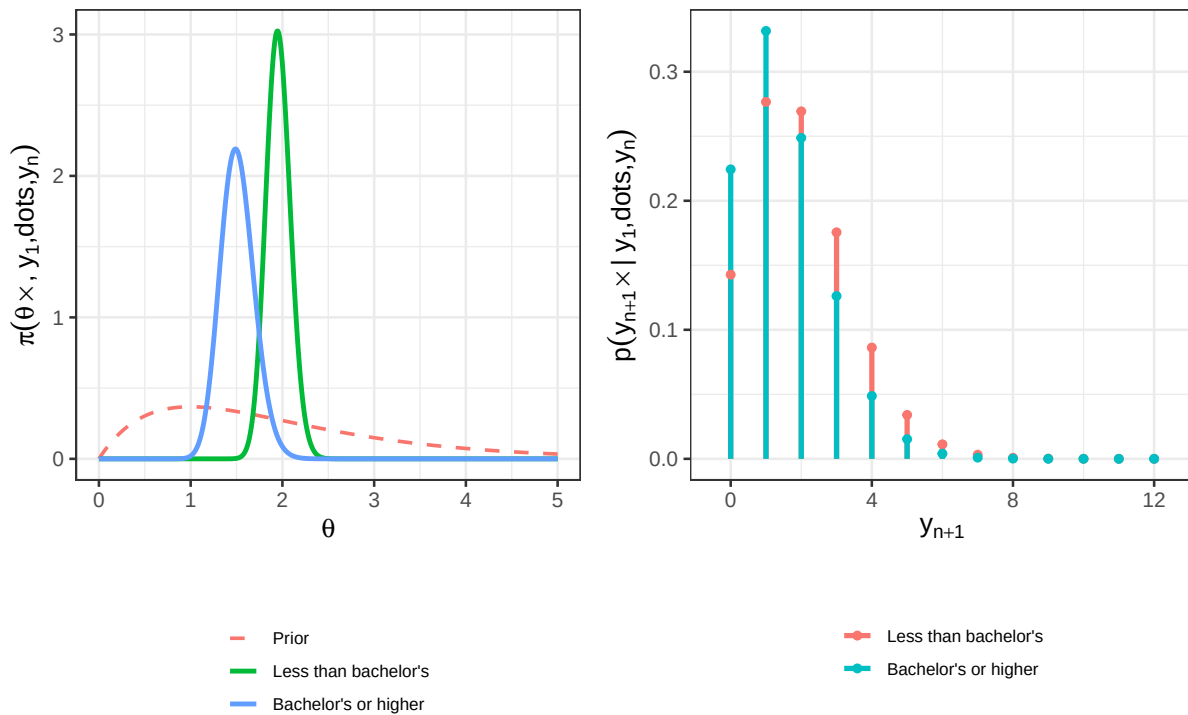
Left: Posterior distributions of mean birth rates; the dashed curve is the common Gamma(2, 1) prior. Right: Posterior predictive distributions for the number of children in each group.
