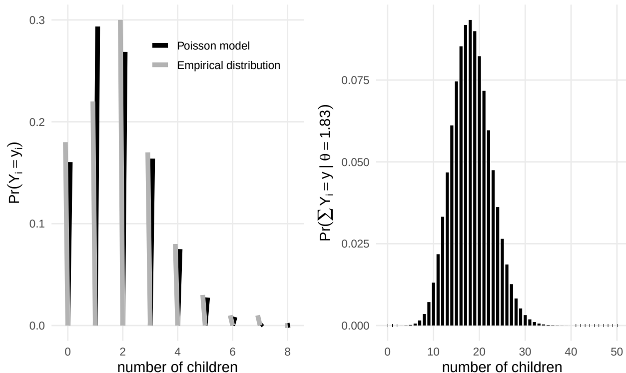
Left: Poisson pmf with mean \theta = 1.83 (black), overlaid with the empirical distribution (grey). Right: The sum of 10 independent Poisson(1.83) variables follows Poisson(18.3). The increased spread illustrates the mean–variance relationship: larger means imply larger variances.
